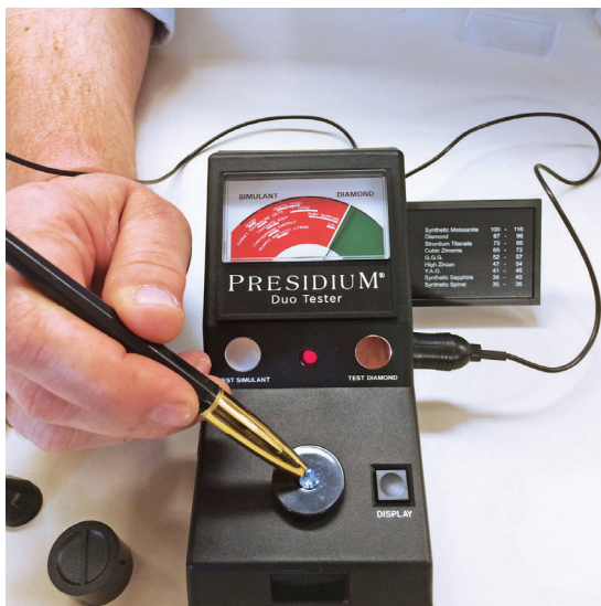
Fig. 2 Duotester in thermotester mode identifies blue diamond correctly as “diamond”
